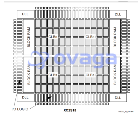
Figure 1: Basic Spartan-II Family FPGA Block Diagram
