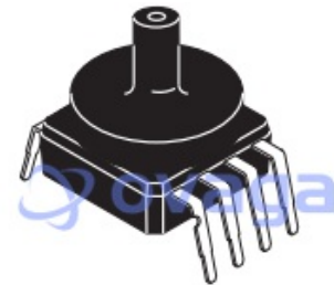
MPXV5010GC7U CASE 482C-03
