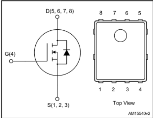
PowerFLAT™ 5x6 Figure 1: Internal schematic diagram
